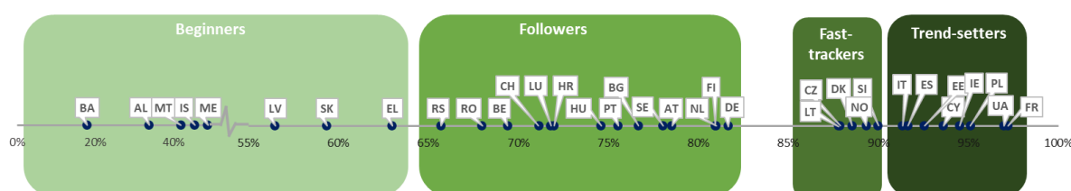
Figure 3: Clustering of the 2022 maturity scores of the participating European countries
