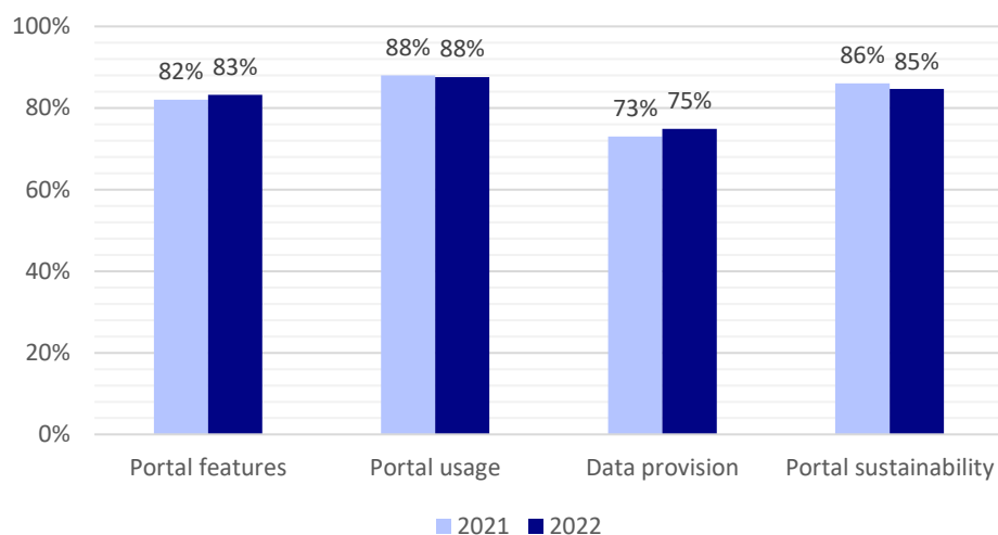
Figure 30: Maturity score per portal indicator compared to last year
